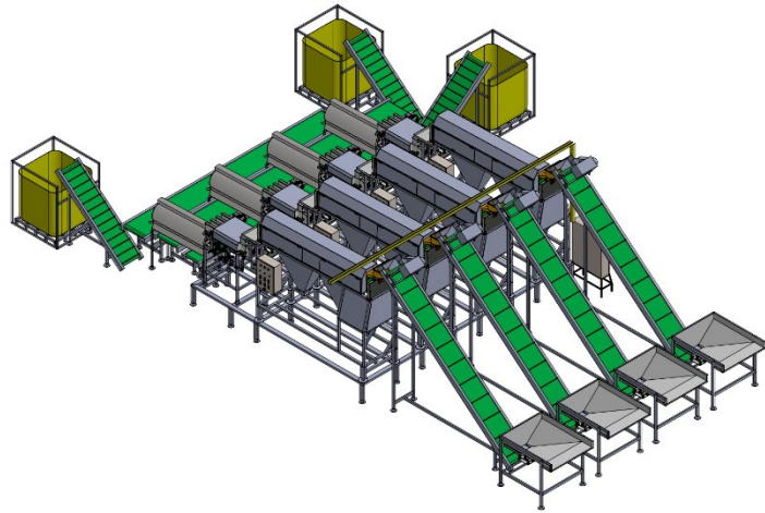
6. MACHINE DE DEPELLICULAGE
